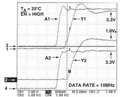
TPC 24. Normal Mode V_{CC1} = 3.3V , V_{CC2} = 1.8V
